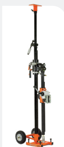
HUSQVARNA DS 50 GYRO ∅ 350 mm, travel length 670 mm, 56 kg.
