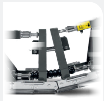
HUSQVARNA BT 90 CROWN INVERT BRACKET 267 mm, maximum angle 15°.
