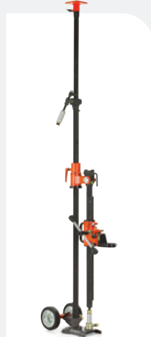
HUSQVARNA DS 40 GYRO ∅ 150 mm, travel length 600 mm, 30 kg.
