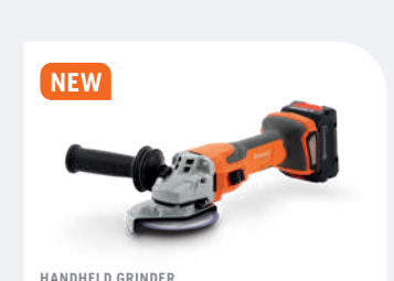
HANDHELD GRINDER HUSQVARNA HG 125 B 1500 W equivalent, grinding width 125 mm, disc speed 11000 rpm, 2.2 Kg (excl. battery). Compatible with all new and existing Bosch Professional 18V tools and chargers.
